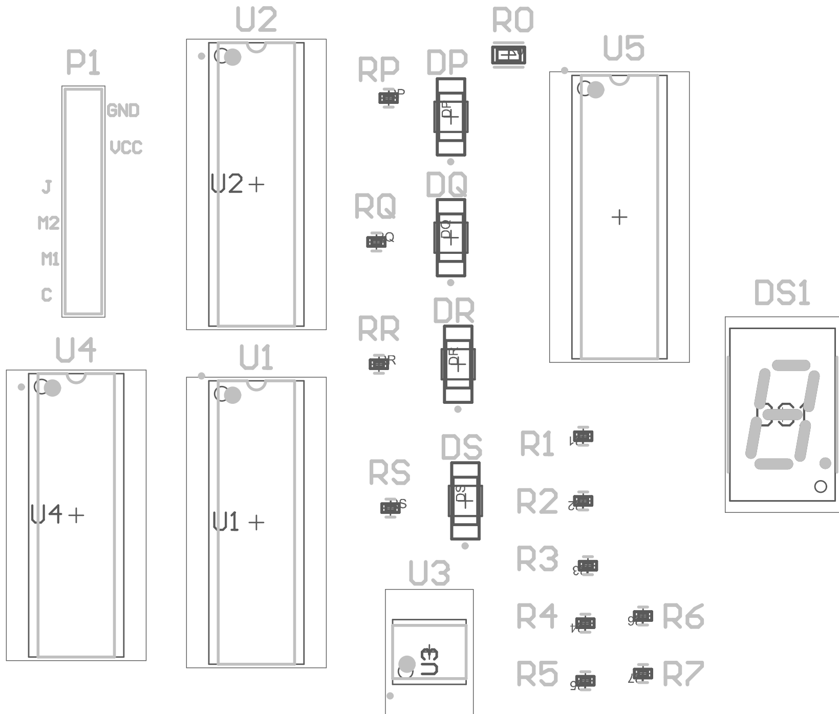
Voting Machine PCB
